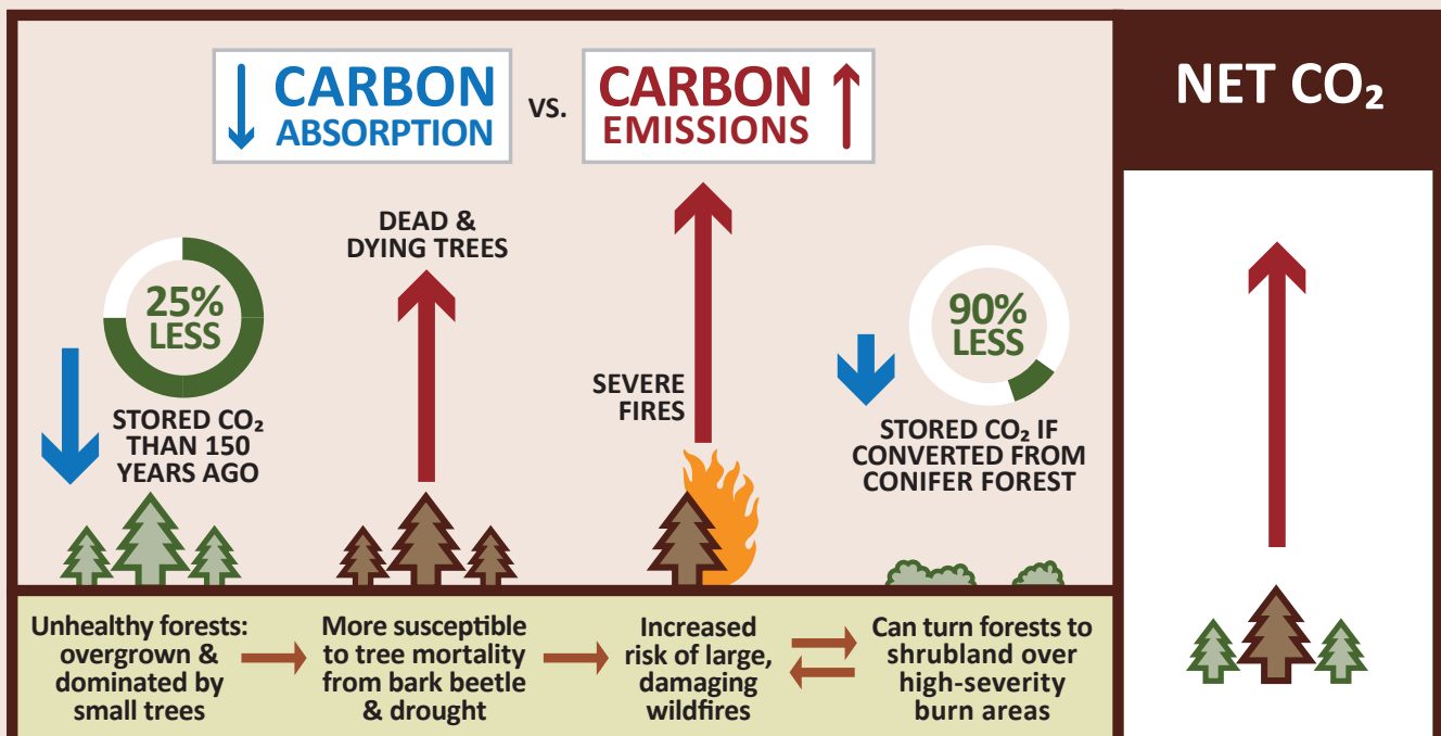
Reduced carbon absorption and storage plus high emissions means many forests are contributing to climate change rather than offsetting it.
